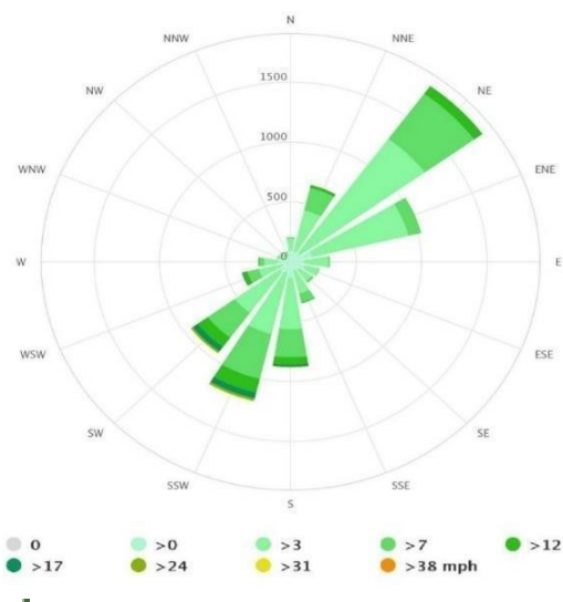
Fig. 4 Wind rose for Tabriz city (meteoblue,2020)
