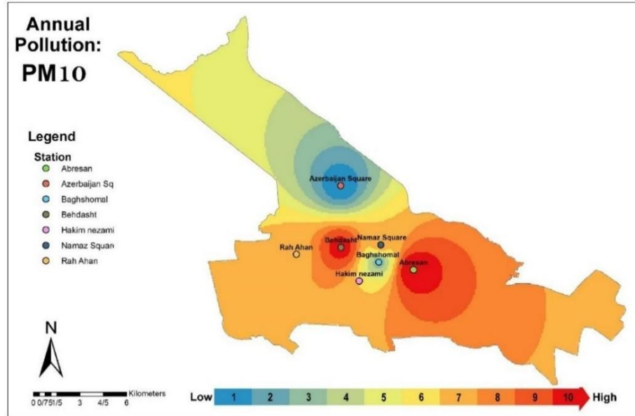
Fig. 11 Tabriz cities annual PM10 pollution index
